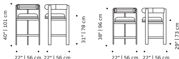
MOULIN bar chair
